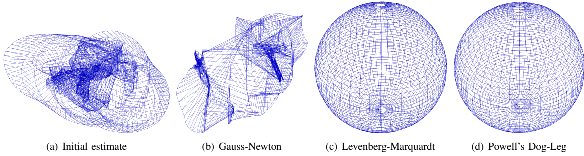
Fig. 5. A representative instance of the sphere2500 6DOF SLAM problem from the batch experiments. (a): The initial estimate for the solution (objective function value 1.221 E8). (b): The solution obtained by Gauss-Newton (3.494 E6). (c): The solution obtained by Levenberg-Marquardt (8.306 E3). (d): The solution obtained by Powell's Dog-Leg (8.309 E3). Note that the objective function value for each of these solutions is within \pm 0.5\% of the median value for the corresponding method given in Table I.
